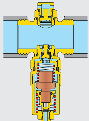
Medium temperature <3°C Valve being drained
